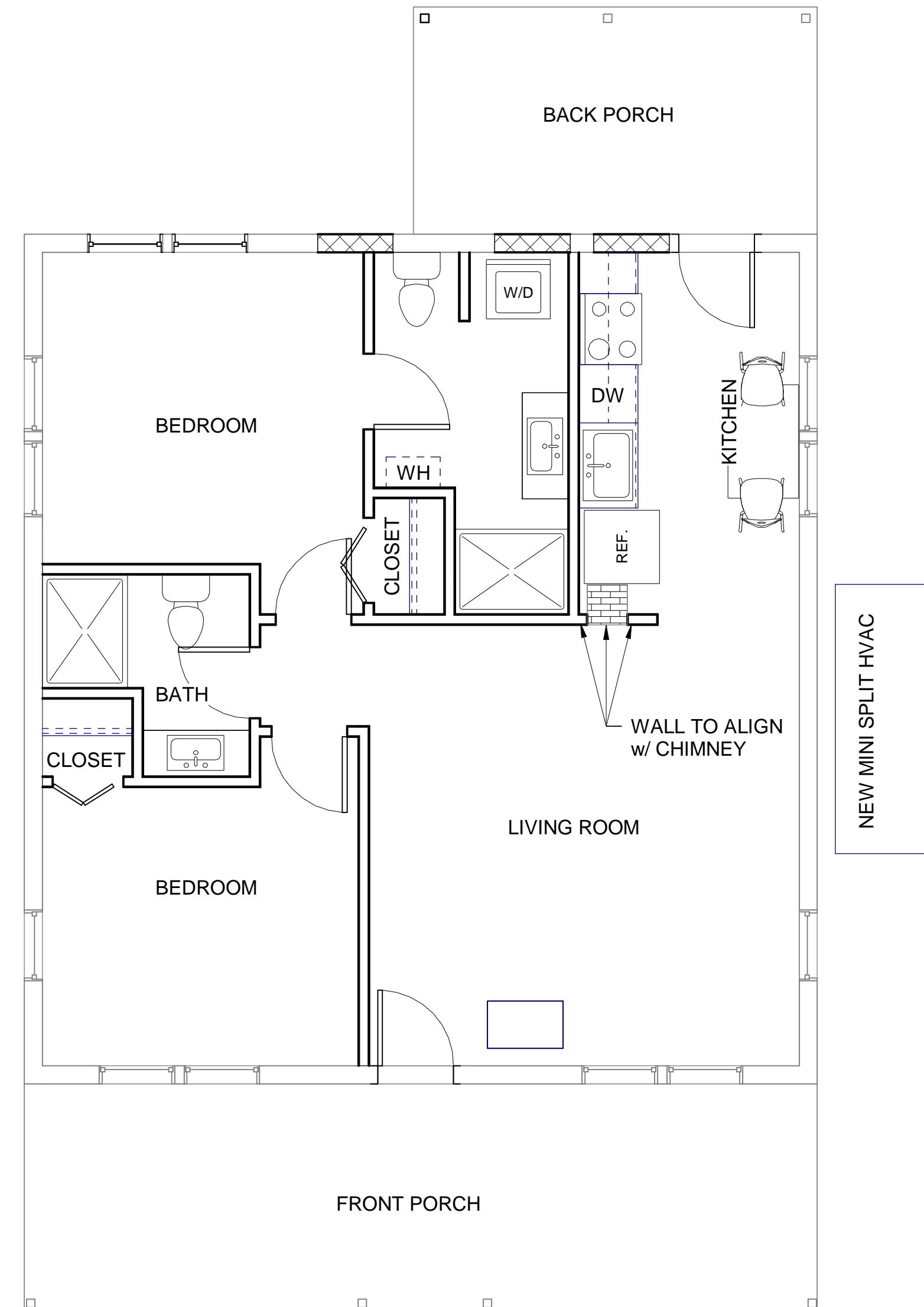
EXTERIOR DIMENSION PLAN
